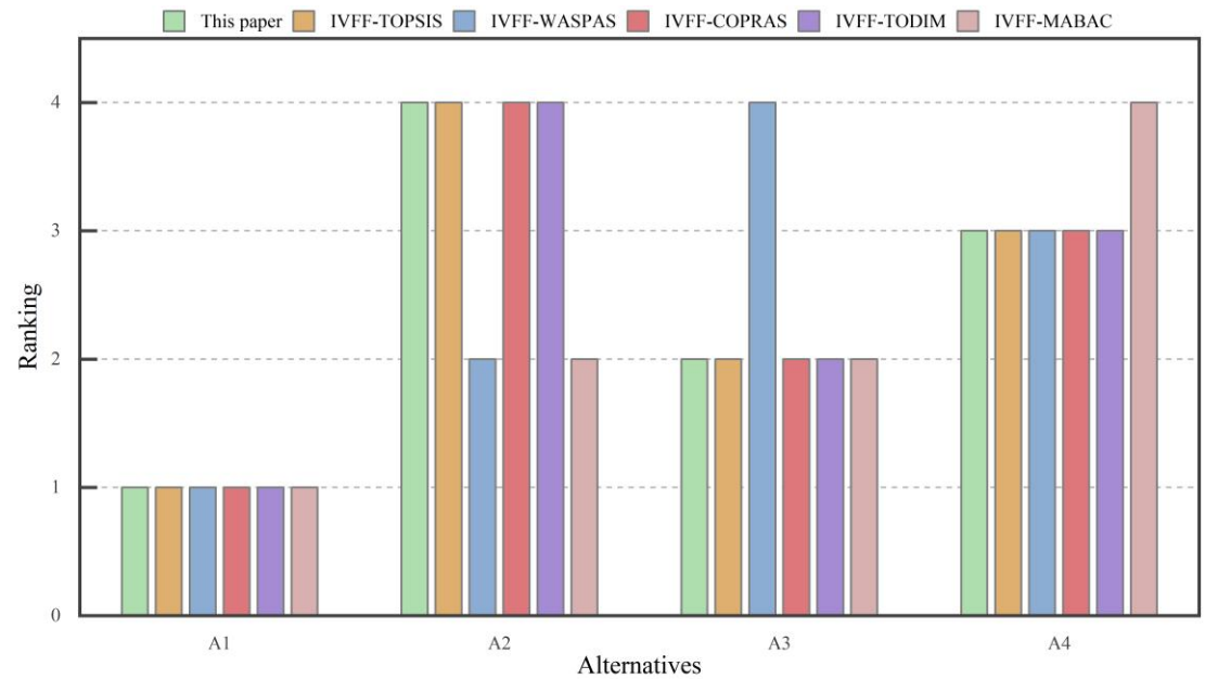
Fig. 5. Ranking results of different MCDM methods.
